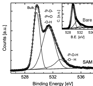
Figure 2. XPS O1s core level spectrum of a bare LSMO substrate (inset) and a C12P LSMO-functionalized substrate (16 h, 0.05 mM in ethanol).
