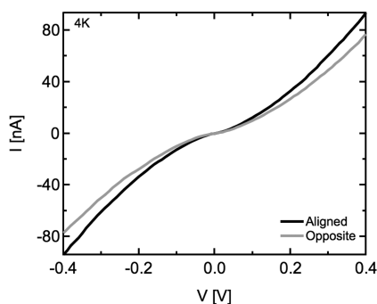
Figure 5. Representative I(V) traces at T = 4 K of Co/C12P/LSMO junctions in the aligned (black) and opposite (gray) magnetic configurations.
